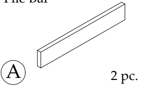
File Bar
